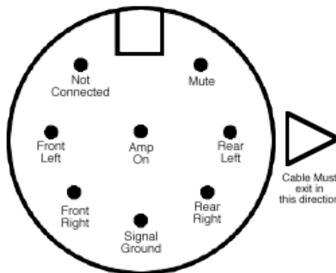
Saab Audio System Pre-Out
