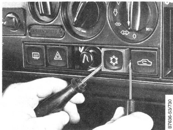
Fig. 2. A/C switch being removed. All square switches pull away from the instrument panel.
