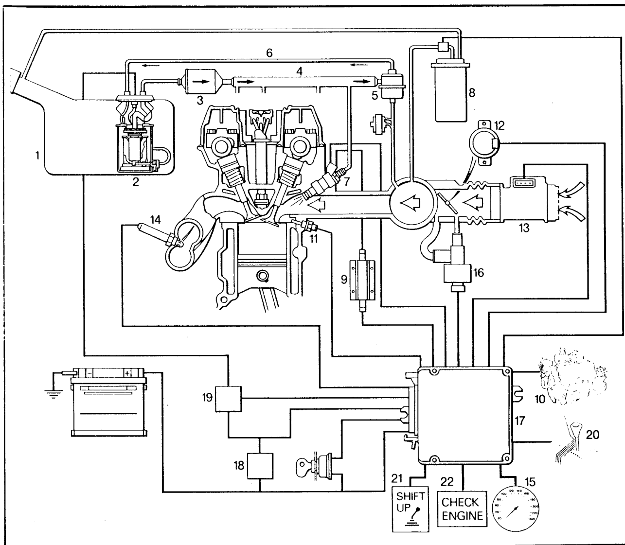
CU14 Fuel-injection system
